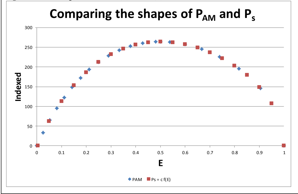
Figure 11 – A Comparison of P_{AM}(E) and P_s(E)
