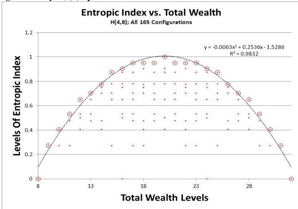
Figure 5 – My H(4,8) space
