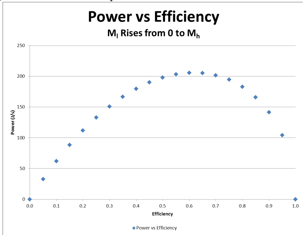
Figure 2 – Power vs Efficiency in Atwood's Machine
