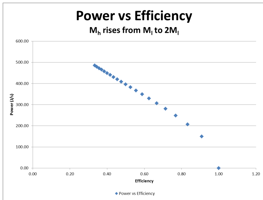
Figure 3 – Power vs Efficiency in Atwood's Machine
