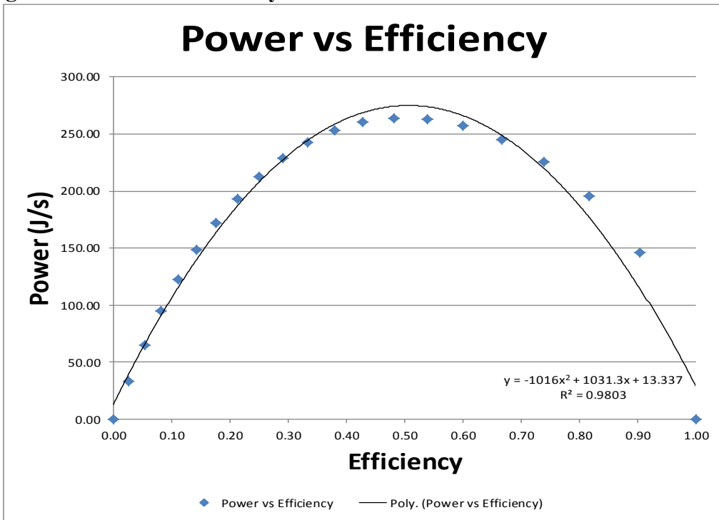
Figure 4 – Power vs Efficiency in Atwood's Machine
